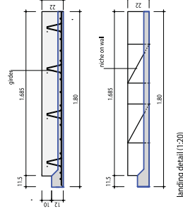
landing slab-wall connection detail(1:20)
